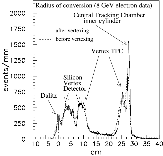
FIG. 2. Vertexed and unvertexed radius of conversion distribution in 8 GeV electron data. The peak at r = 0 labeled 'Dalitz' is due to \pi^0 \rightarrow e^+ e^- \gamma decays and \gamma^* \rightarrow e^+ e^- events. The 2 \text{ cm} < r < 30 \text{ cm} data selection requirement has been released in this plot.
